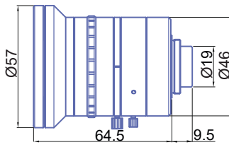
GM12HR30528MCN
