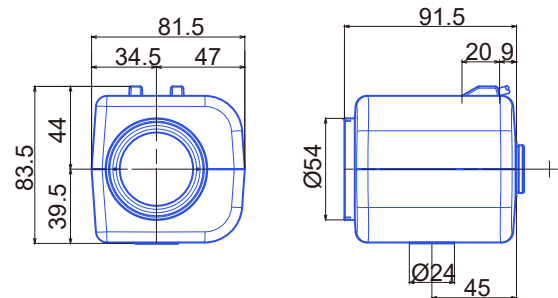
GAZMPDN280800M
