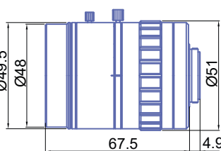
GM12HR41616MCN
