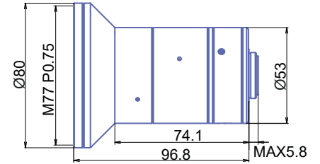
GM12HR58018MCN
