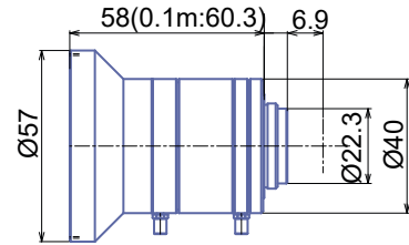
GMTHR48014MCN-1
