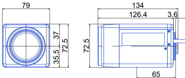
GAZMP280136M
