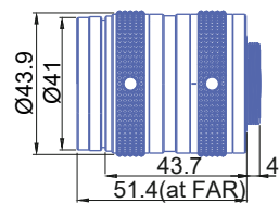
GM12HR42516MCN
