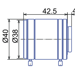
GMTHR42514MCN
