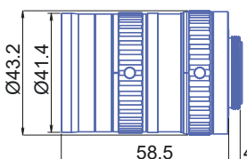
GM12HR35018MCN
