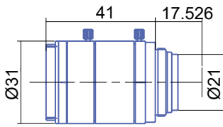
GM6HR38014MCN
