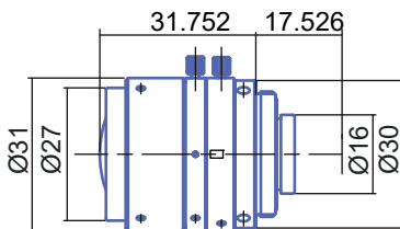
GMTHR23514MCN
