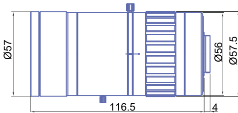
GM12HR57518MCN
