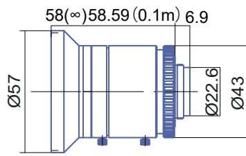
GMTHR41614MCN
