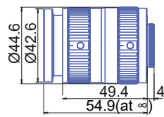
GM12HR52514MCN
