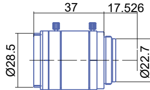
GM6HR31214MCN
