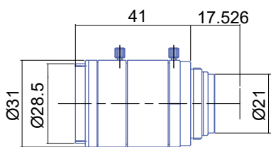
GMHR32514MCN-1
