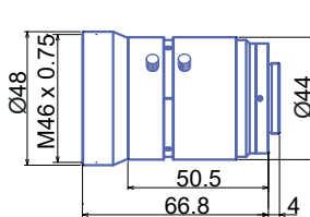
GM12HR312514MCN-1
