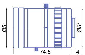
GM12HR42016MCN
