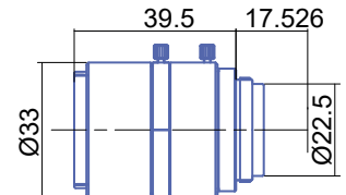
GM6HR32514MCN
