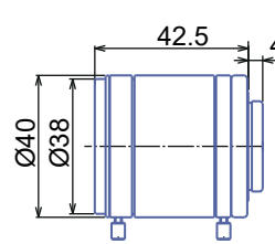
GMTHR43514MCN
