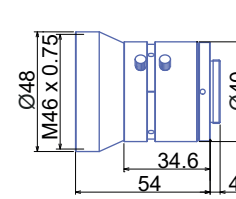
GM12HR39014MCN-1
