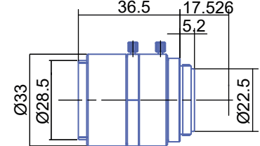
GMTHR35028MCN-1
