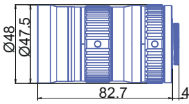
GM12HR551618MCN
