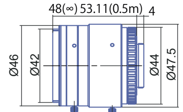
GMTHR412514MCN-1
