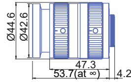
GM12HR53514MCN
