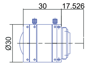
GMTHR36014MCN
