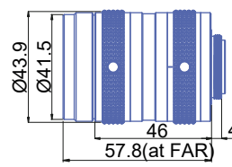
GM12HR30528MCN
