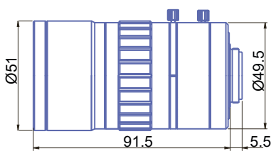
GM12HR57518MCN
