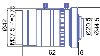
GM12HR31214MCN
