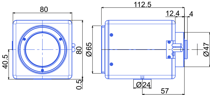
GAZMPDN42465M
