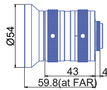
GM12HR30528MCN
