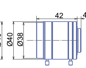
GMTHR41614MCN
