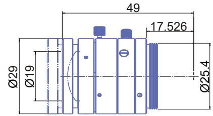
GMTHR35028MCN-1
