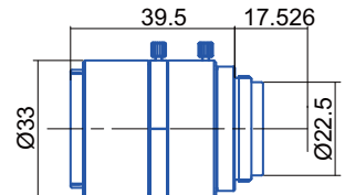
GM6HR32514MCN
