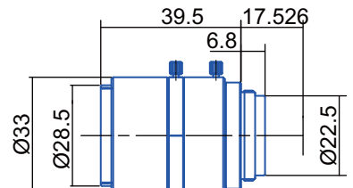
GMHR32514MCN-1
