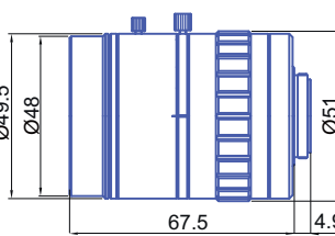
GM12HR41616MCN
