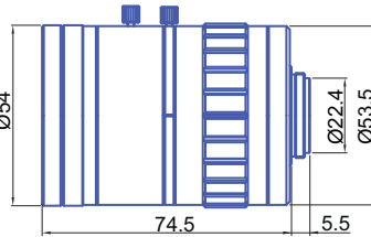
GM12HR41216MCN
