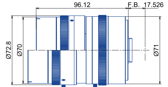
GMHR62409MCN
