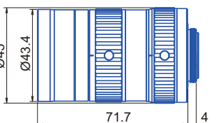
GM12HR37520MCN
