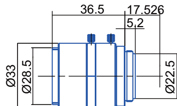
GMHR31614MCN-1
