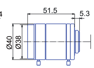
GMTHR412514MCN-1
