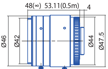
GMTHR45014MCN
