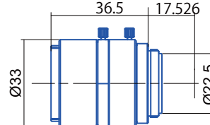
GM6HR31614MCN
