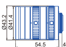
GM12HR32514MCN
