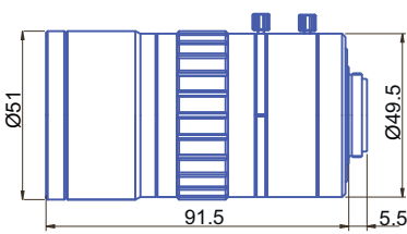
GM12HR57518MCN
