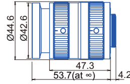
GM12HR53514MCN
