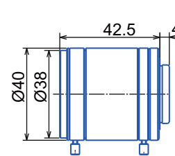
GMTHR42514MCN
