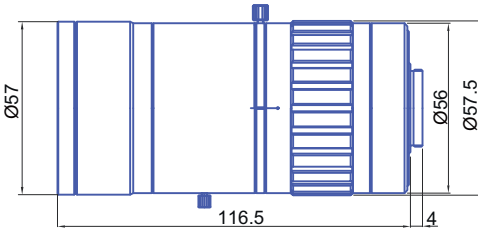
GM12HR57518MCN
