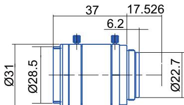
GMHR31214MCN-1
