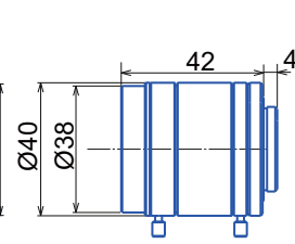
GMTHR41614MCN
