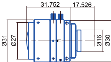
GMTHR23514MCN
