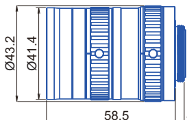
GM12HR35018MCN
