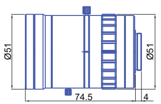
GM12HR42016MCN
