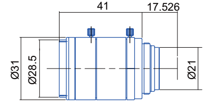
GMHR38014MCN-1
